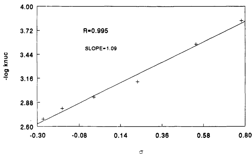
Figure 2. Hammett plot for the reaction of G_1 - N -phenylhydroxylamines with methyl 3-nitrobenzenesulfonate at 29.5 °C in methanol- d_4 .
