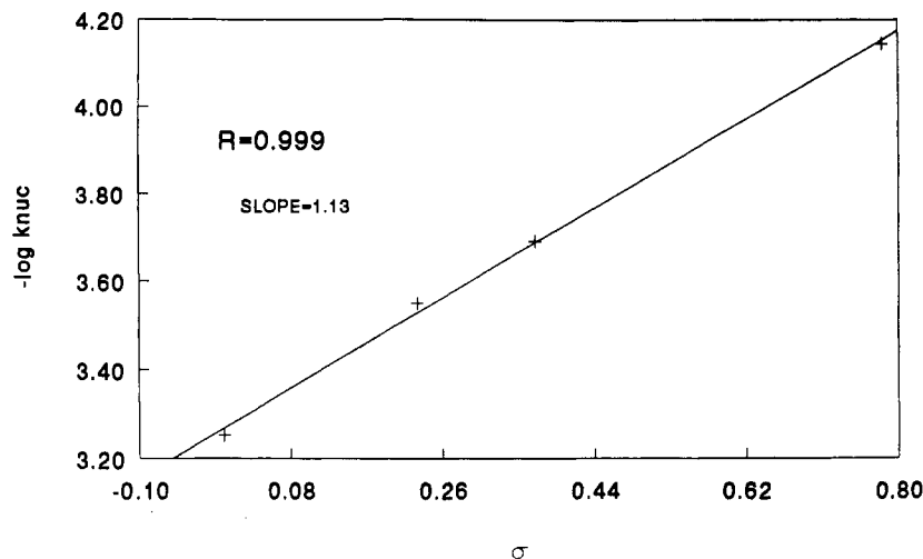
Figure 1. Hammett plot for the reaction of G_1 - N -methylanilines with methyl 3-nitrobenzenesulfonate in methanol- d_4 at 29.5 °C.
